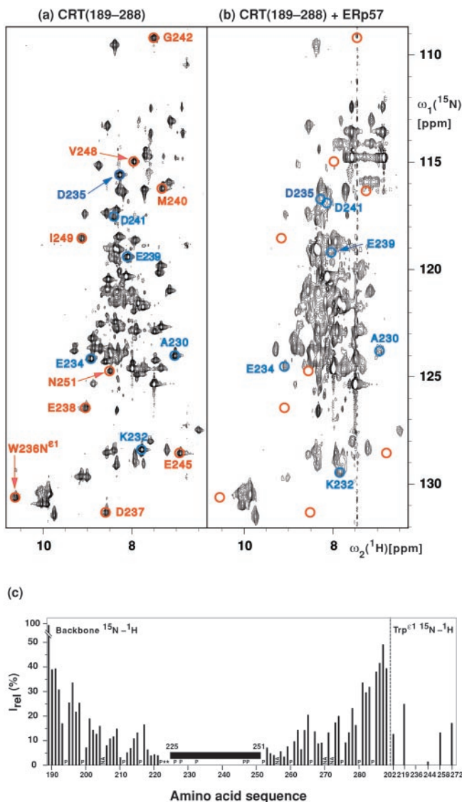
Fig. 2. (a and b) ^{15}\text{N} - ^1\text{H} correlation NMR spectra used to delineate the surface areas of CRT(189–288) that interact with ERp57. These spectra contain peaks corresponding to backbone amide ^{15}\text{N} - ^1\text{H} groups and, in the lower left, indole ^{15}\text{N} - ^1\text{H} groups of tryptophyl residues. Color-coded peaks indicate outstandingly large effects from ERp57 interactions: Blue circles identify cross peaks with chemical shift differences of more than 0.2 ppm along the ^{15}\text{N} dimension between free and ERp57-bound CRT(189–288). Red circles identify cross-peak positions in free CRT(189–288) for which no counterpart could be observed in the spectrum of the complex. The color-coded cross peaks are labeled with the sequence-specific resonance assignments. (a) [ ^{15}\text{N} , ^1\text{H} ]TROSY spectrum of free ^{15}\text{N} , ^2\text{H} -labeled CRT(189–288) (protein concentration = 0.4 mM, polarization transfer time = 5.4 ms, data size 200 \times 1,024 complex points, zero-filling to 512 \times 2,048 points, t_{1,\text{max}} = 88 ms, t_{2,\text{max}} = 98 ms, total measuring time 2 h). (b) [ ^{15}\text{N} , ^1\text{H} ]TROSY spectrum of a solution of ^{15}\text{N} , ^2\text{H} -labeled CRT(189–288) and unlabeled ERp57 [protein concentrations of 0.14 mM for ^{15}\text{N} , ^2\text{H} -labeled CRT(189–288) and 0.38 mM for ERp57, polarization transfer time = 3.4 ms, data size 100 \times 1,024 complex points, zero-filling to 512 \times 2,048 points, t_{1,\text{max}} = 44 ms, t_{2,\text{max}} = 98 ms, total measuring time 24 h]. (c) Plot of the relative peak intensities, I_{\text{rel}} , of the [ ^{15}\text{N} , ^1\text{H} ]TROSY cross peaks in the CRT(189–288)/ERp57 complex and free CRT(189–288) versus the amino acid sequence of CRT(189–288). The Trp indole cross peaks are listed separately on the right. The black horizontal bar spanning the polypeptide segment 225–251 indicates that for these residues the cross peaks in the complex have either large chemical shift differences ( > 0.2 ppm along the ^{15}\text{N} dimension) or very small signal intensities [ < 3\% of the intensity in free CRT(189–288)] (see text). P designates proline residues, NA stands for residues for which no resonances could be assigned, and * indicates residues for which no reliable data could be measured because of spectral overlap.
